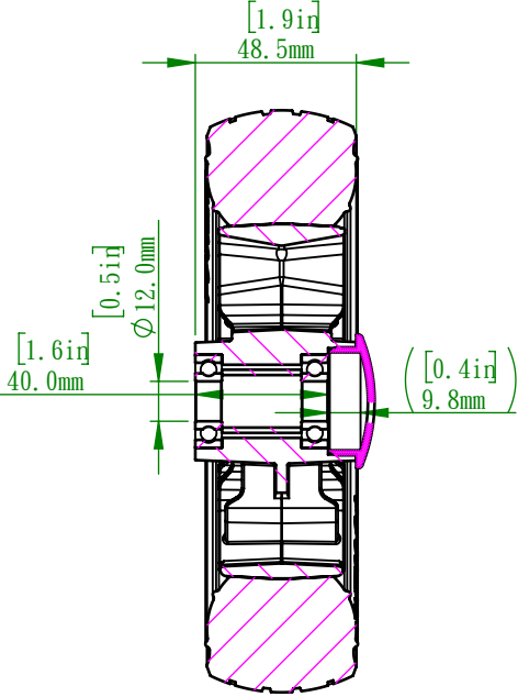
SECTION C-C
