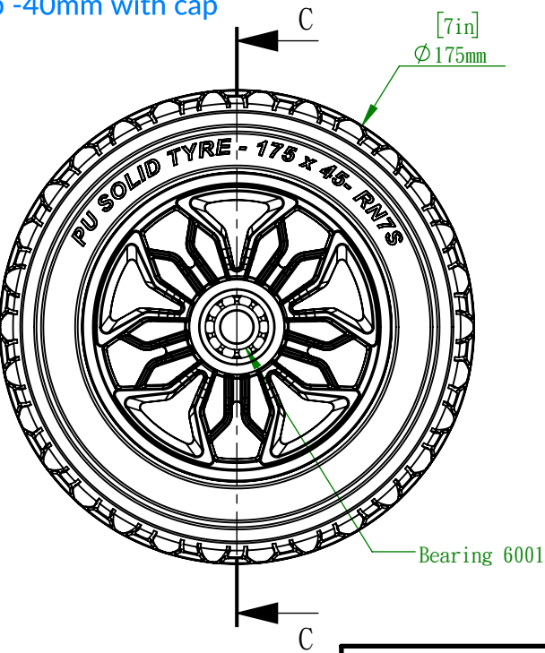
C Type - Eccentric Hub -40mm with cap
