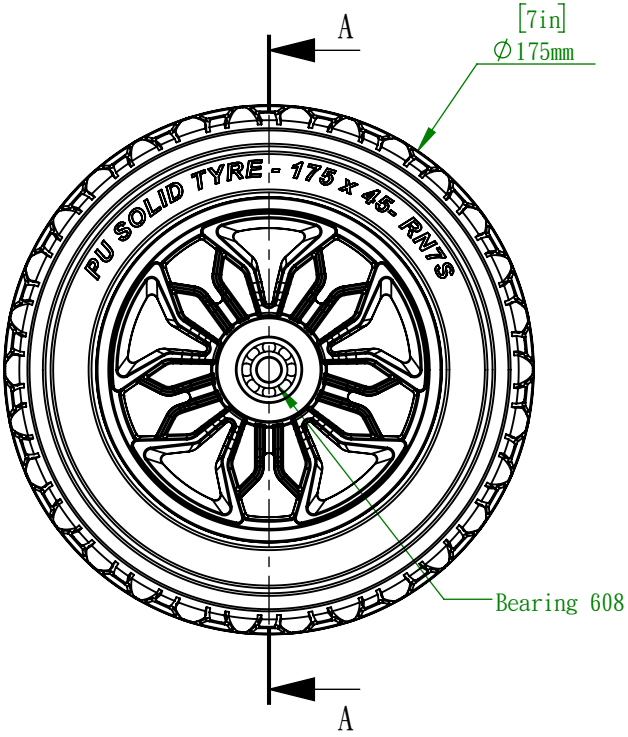
A Type - Centric Hub -60mm (Bearing 608)
